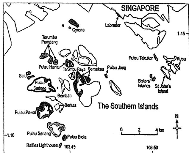
Shaded area = coral reef
